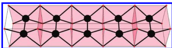
Chart 1. View of a Technetium Dichloride Chain Along the c Axis of the Unit Cell 2
