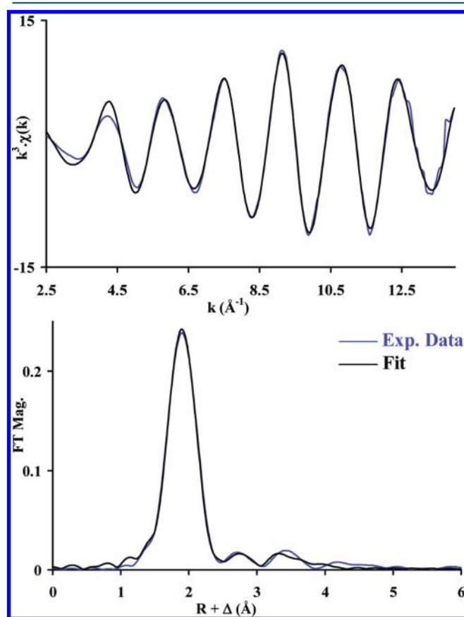
Figure 4. Fitted experimental k^3 EXAFS spectra (top) and Fourier transform of k^3 EXAFS spectra (bottom) of \text{TcCl}_2 . Adjustment between k = 2.5 – 14 \text{ \AA}^{-1} . Experimental data (blue) and fit (black).
